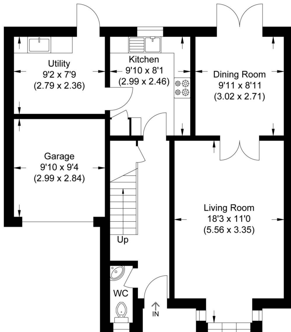
Ground Floor
