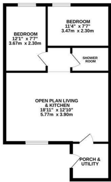
LOWER FLOOR (APARTMENT) 517 sq.ft. (48.0 sq.m.) approx.
