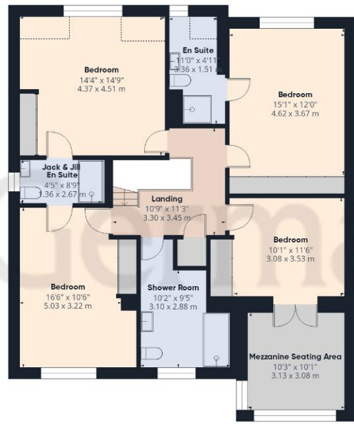
Floor 1
