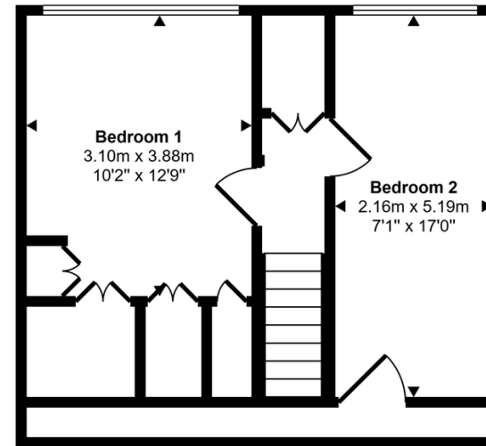
First Floor Approx 37 sq m / 401 sq ft
