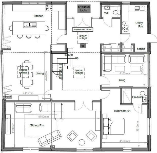
Proposed ground floor plan (Barn 01)
