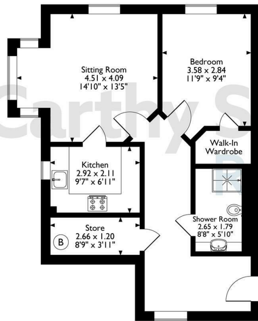
The position & size of doors, windows, appliances and other features are approximate only. © ehouse. Unauthorised reproduction prohibited. Drawing ref. dij/8660980/DST.
