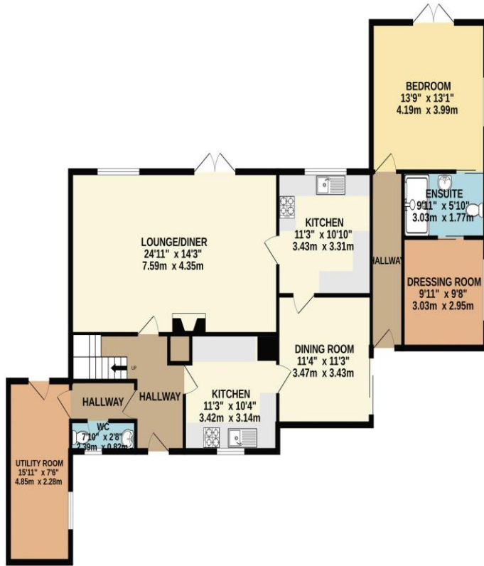
GROUND FLOOR 1363 sq.ft. (126.6 sq.m.) approx.
