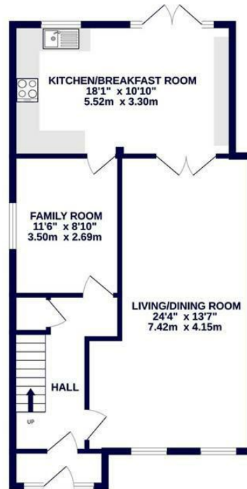
GROUND FLOOR 698 sq.ft. (64.8 sq.m.) approx.
