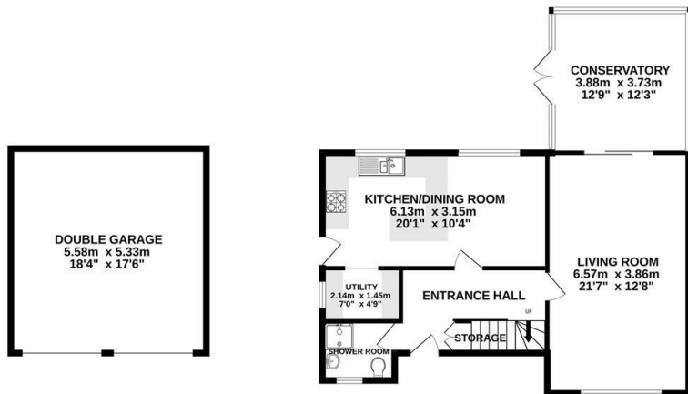
GROUND FLOOR 104.5 sq.m. (1125 sq.ft.) approx.
