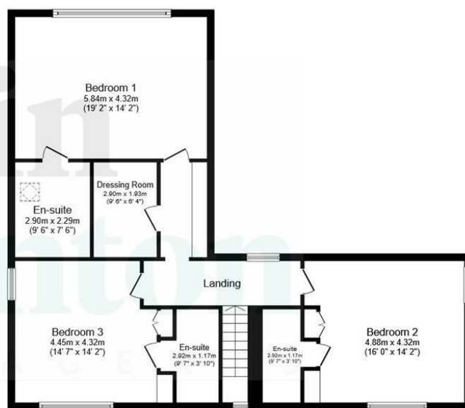
First Floor Floor area 102.3 sq.m. (1,101 sq.ft.)
