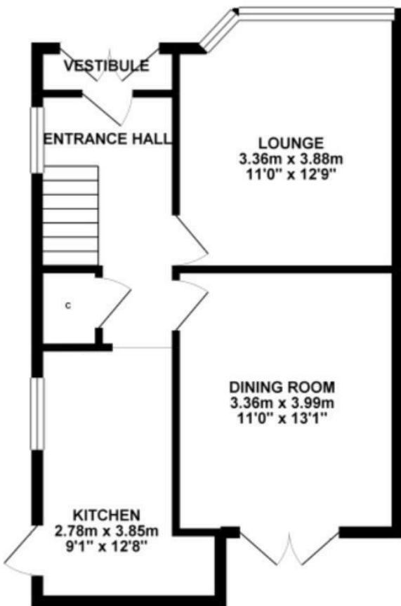
GROUND FLOOR 44.43 sq. m. ( 478.22 sq. ft. )
