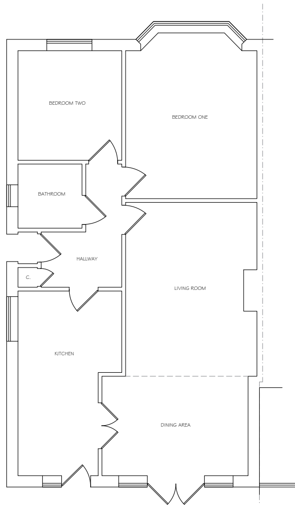
Existing Floor Plan 1:100 @ A3
