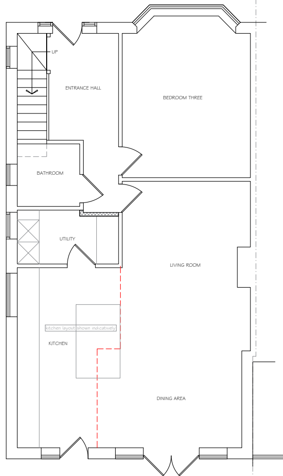
Proposed Ground Floor Plan 1:100 @ A3
