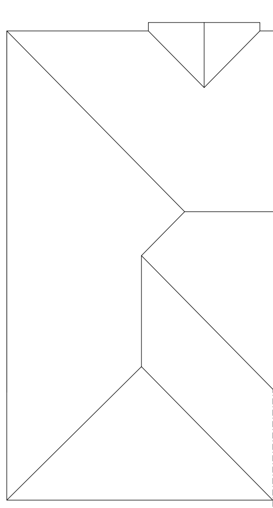
Existing Roof Plan 1:100 @ A3
