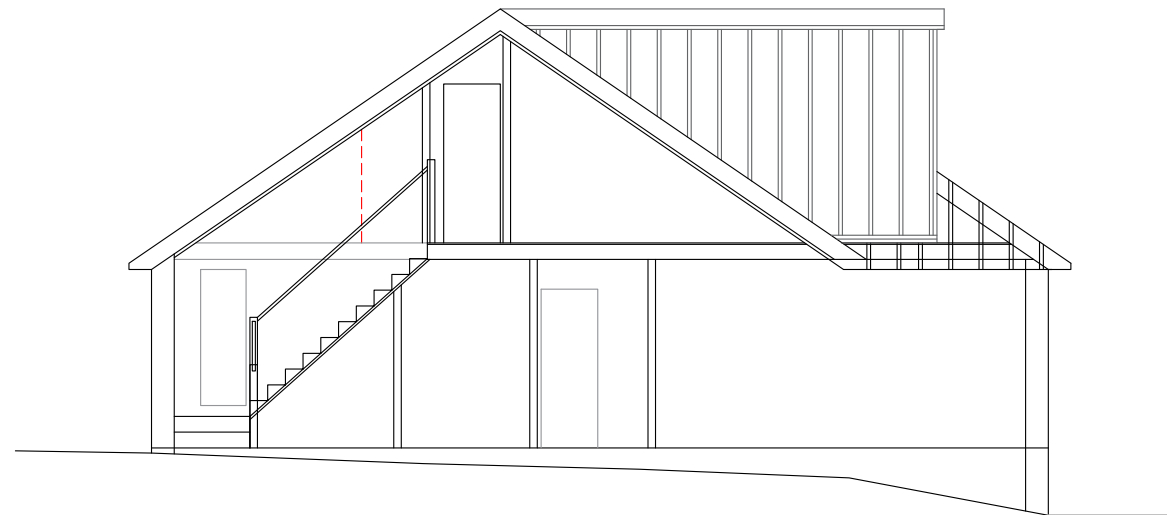
Proposed Section 1:100 @ A3
