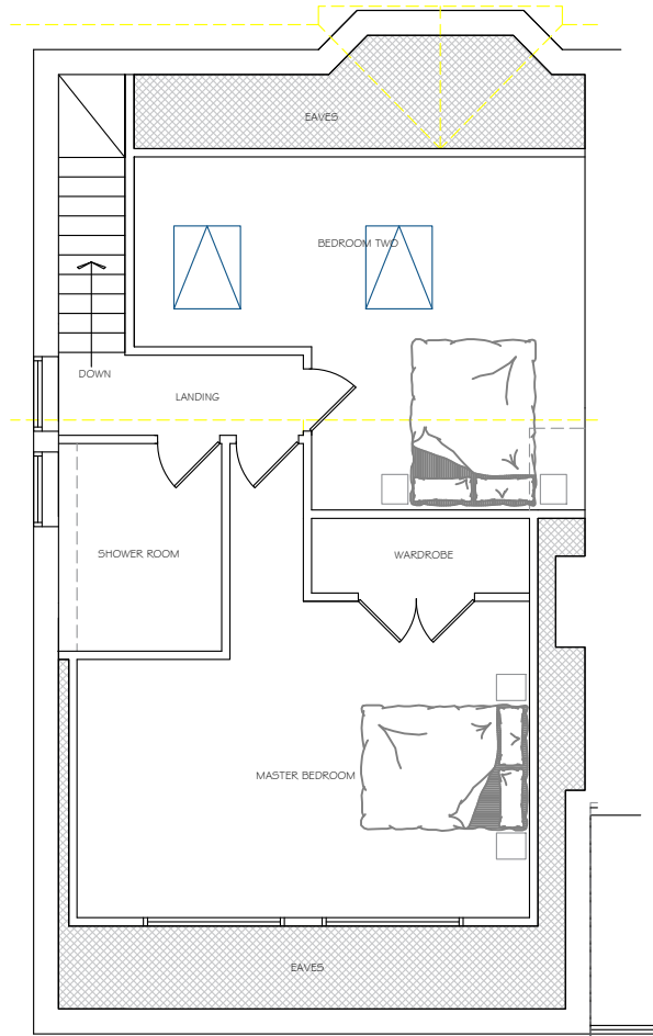
Proposed First Floor Plan 1:100 @ A3
