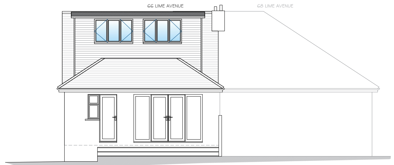
Existing Rear Elevation 1:100 @ A3
