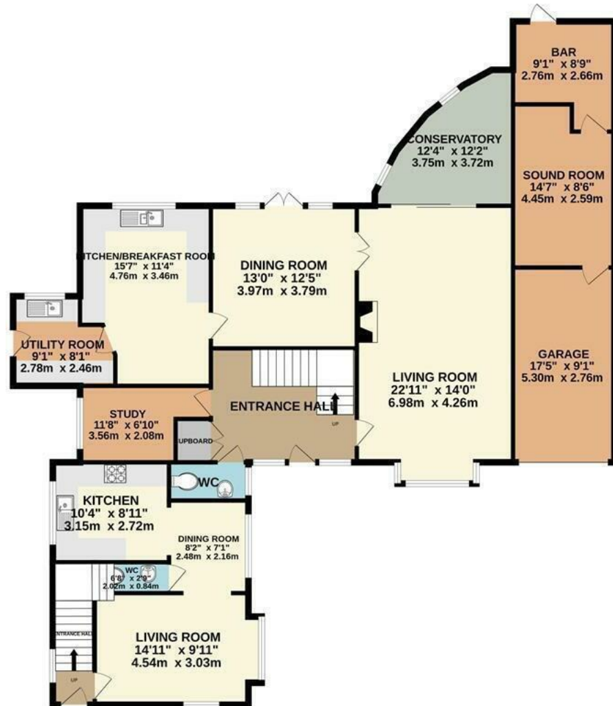
GROUND FLOOR 1788 sq.ft. (166.1 sq.m.) approx.
