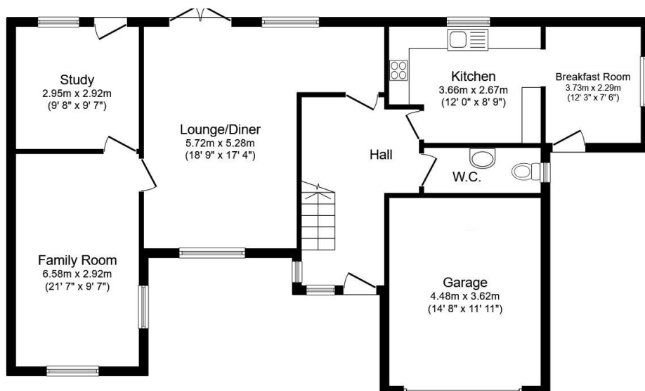
Ground Floor Floor area 94.7 sq.m. (1,019 sq.ft.)
