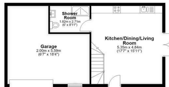
Ground Floor, Second Property Approx. 56.4 sq. metres (606.6 sq. feet)
