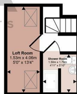
Second Floor Approx 13 sq m / 135 sq ft
