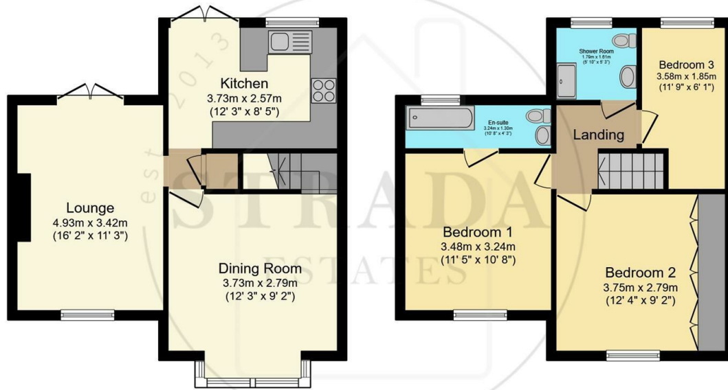
Ground Floor Floor area 43.2 sq.m. (465 sq.ft.)
