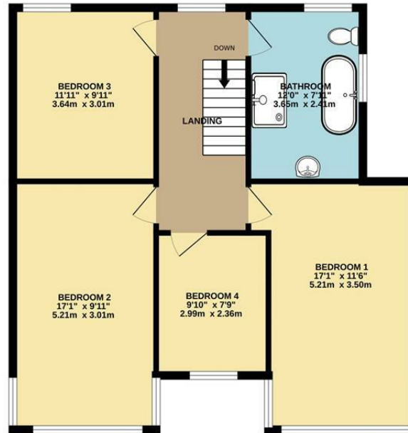
1ST FLOOR 734 sq.ft. (68.2 sq.m.) approx.
