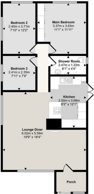
Floorplan
