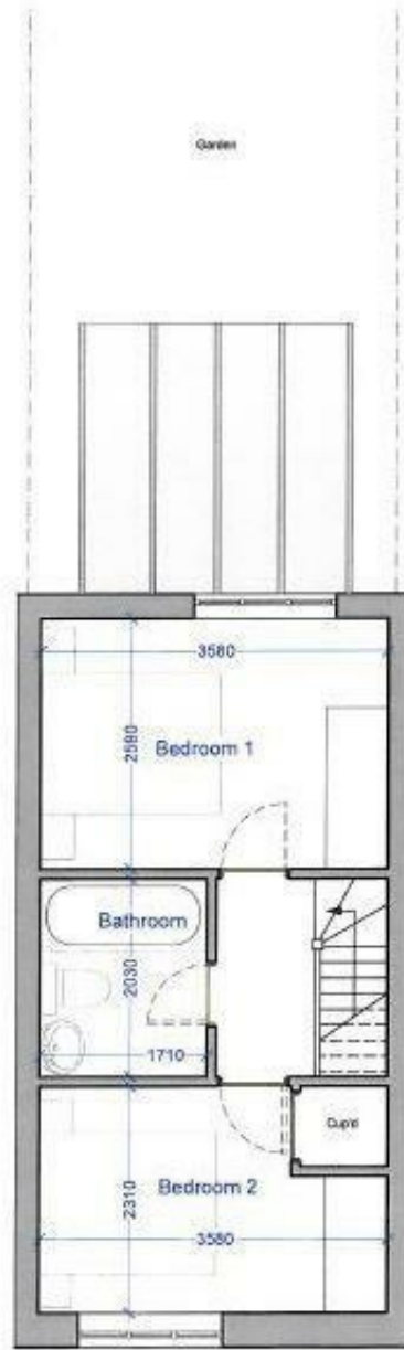
FIRST FLOOR PLAN SCALE 1:50
