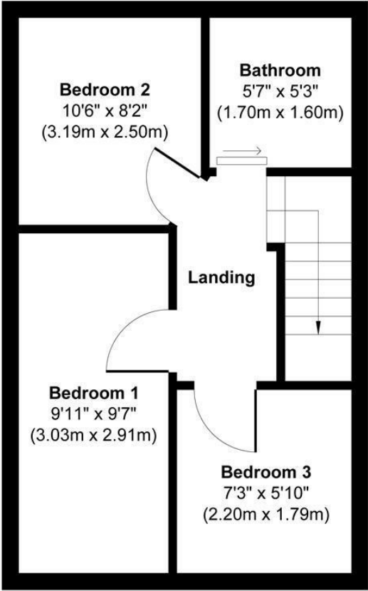
First Floor Approximate Floor Area 287 sq. ft (26.64 sq. m)
