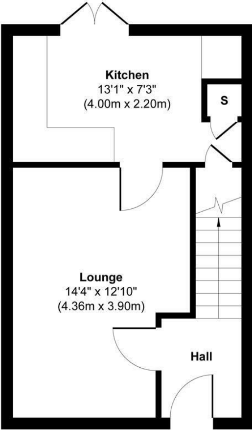
Ground Floor Approximate Floor Area 287 sq. ft (26.64 sq. m)
