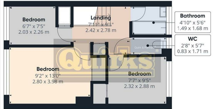
Floor 1 Building 1
