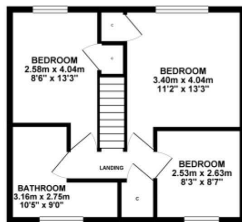
1ST FLOOR 40.80 sq. m. ( 439.20 sq. ft. )
