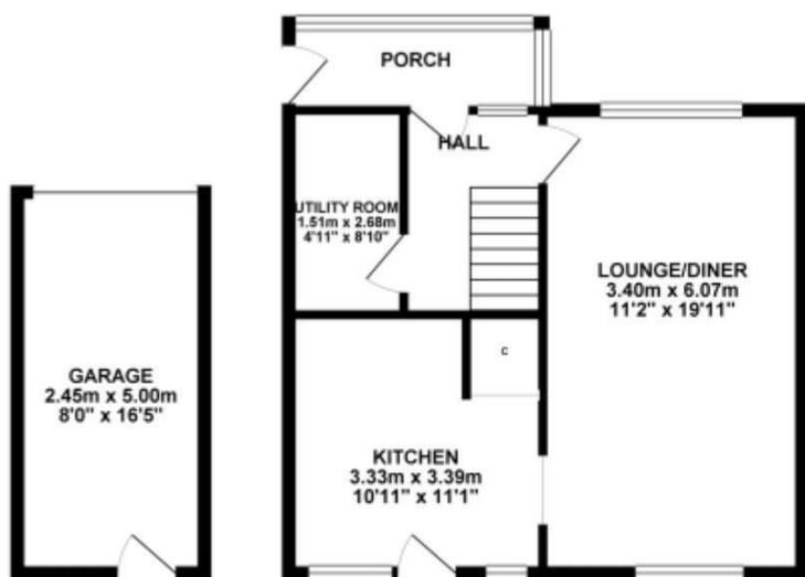
GROUND FLOOR 56.86 sq. m. ( 611.99 sq. ft. )
