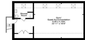
First Floor Garage
