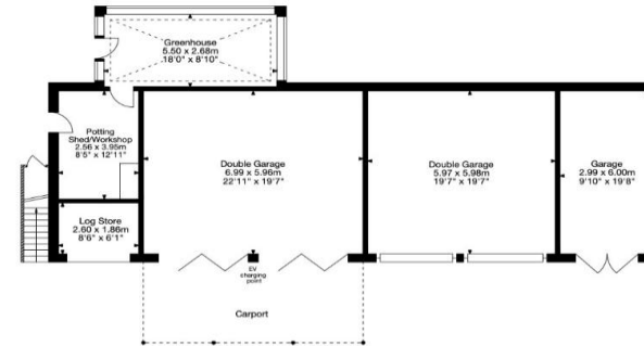
Ground Floor Garage
