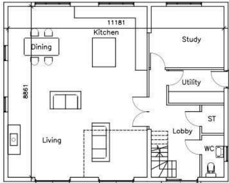
Proposed ground floor plan 198m 2 Total GIA 0 3m
