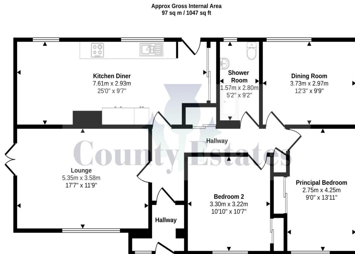
Floorplan
