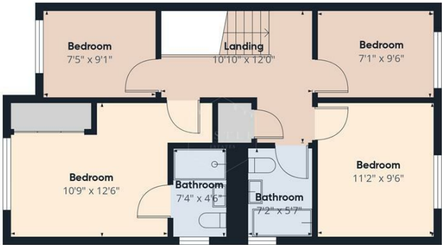
Floor 1 Building 1
