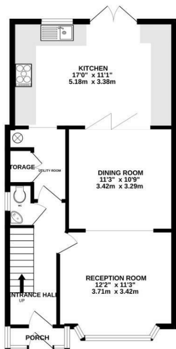
GROUND FLOOR 576 sq.ft. (53.5 sq.m.) approx.
