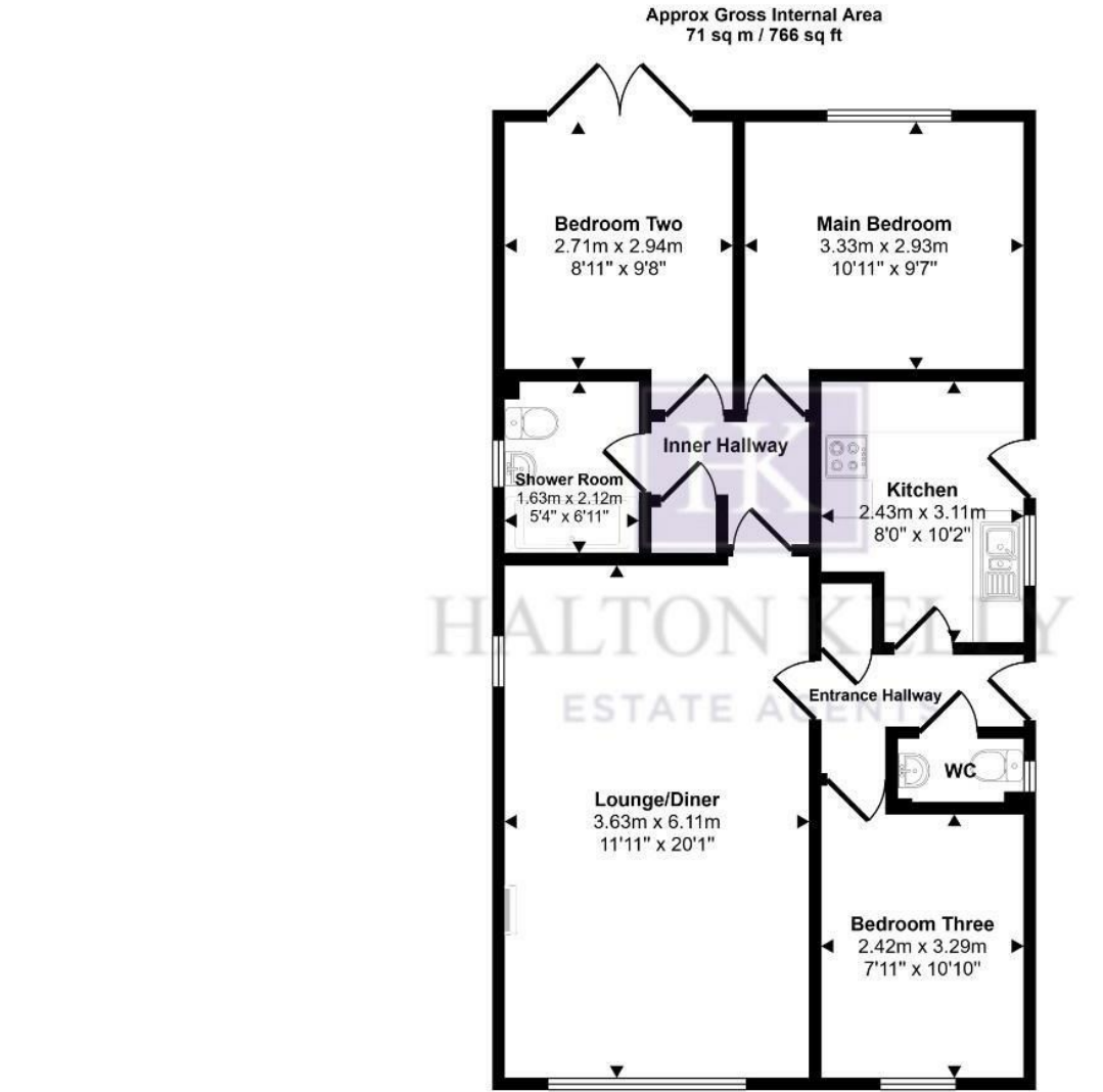
Floorplan
