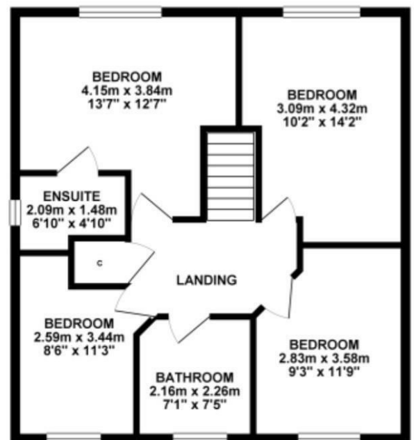
1ST FLOOR 57.16 sq. m. ( 615.31 sq. ft. )
