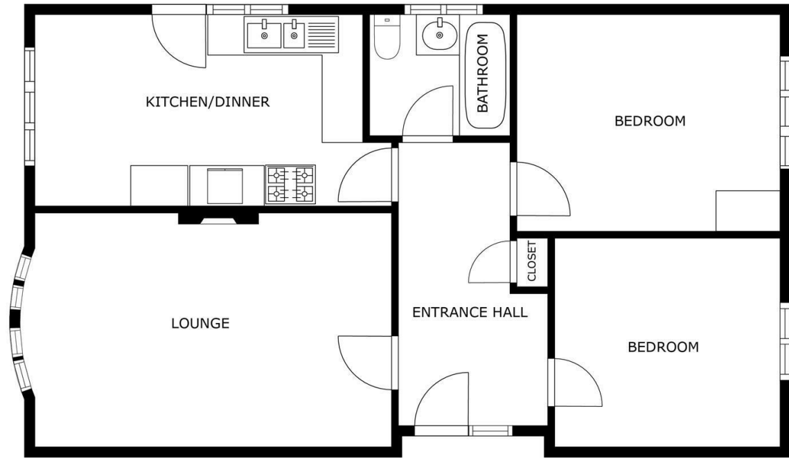
FLOOR PLAN
