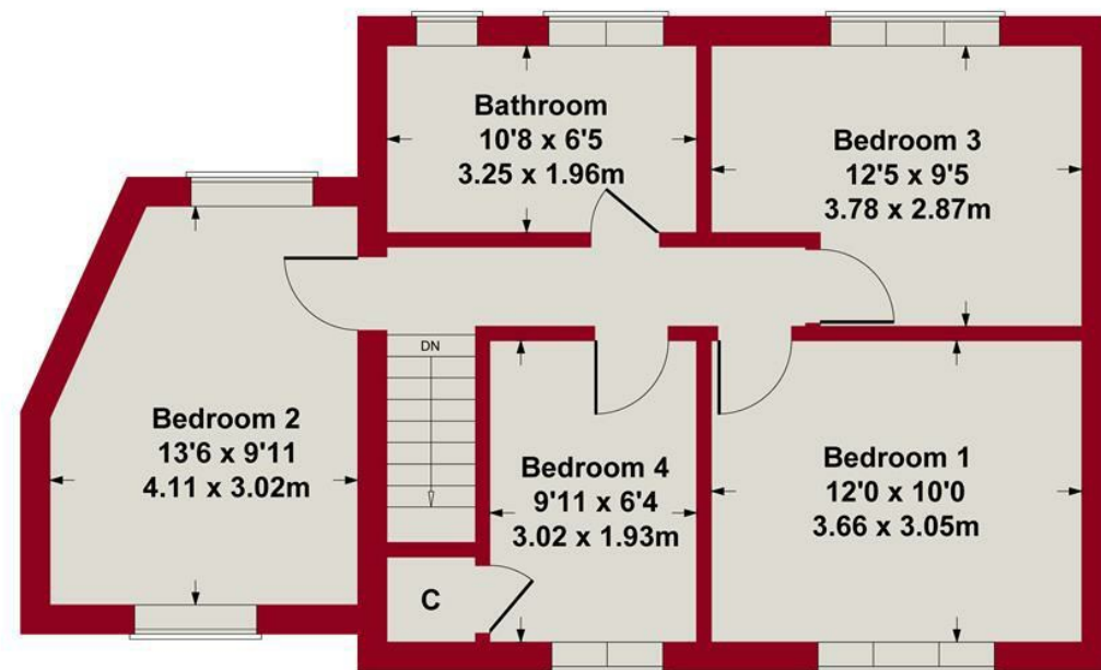
FIRST FLOOR
