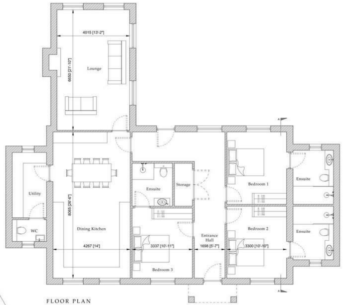
FLOOR PLAN
