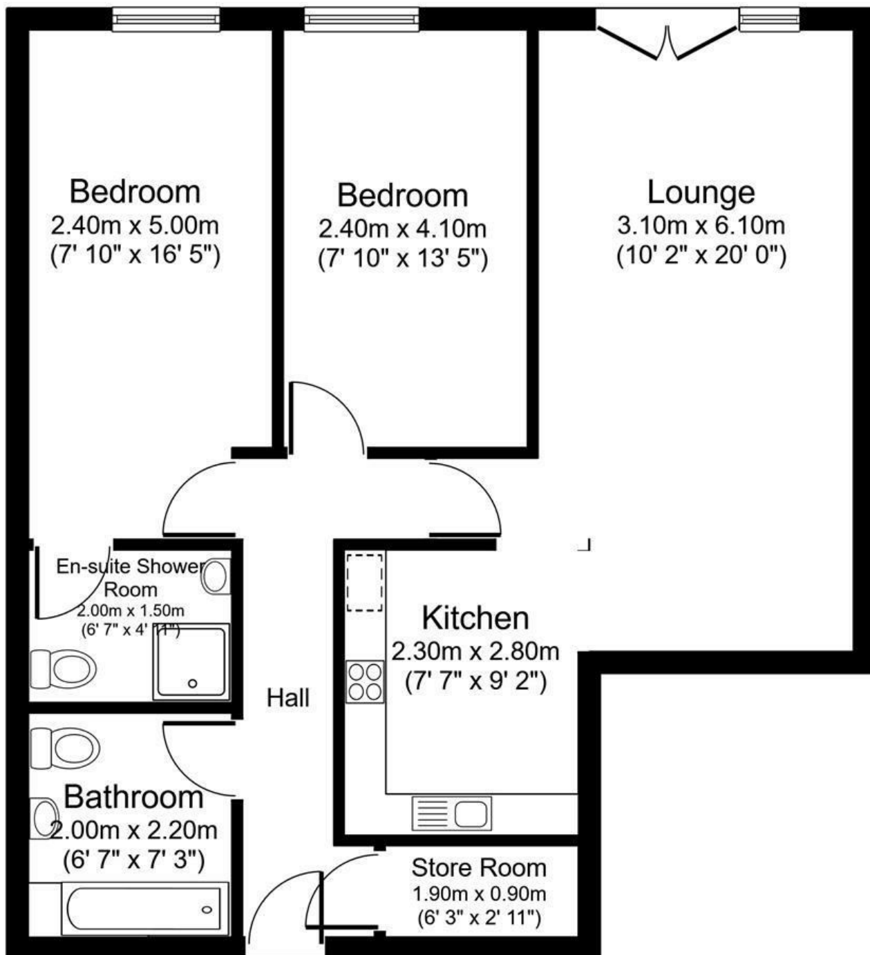
Floor Plan
