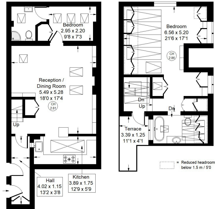
Ground Floor and First Floor
