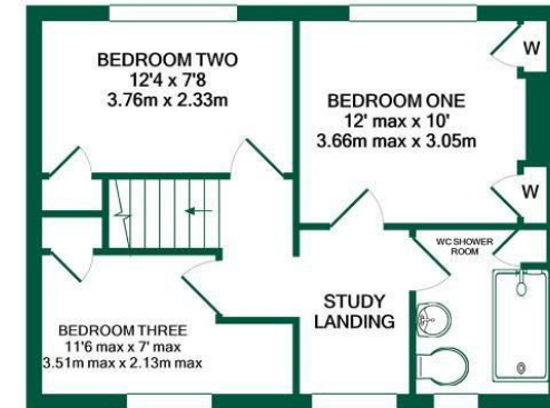
FIRST FLOOR APPROX. FLOOR AREA 438 SQ.FT. (40.7 SQ.M.)
