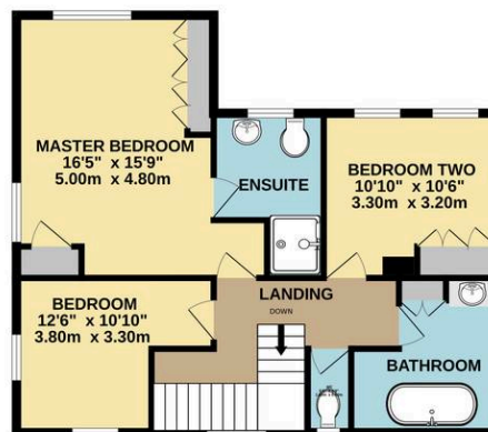
1ST FLOOR 681 sq.ft. (63.2 sq.m.) approx.
