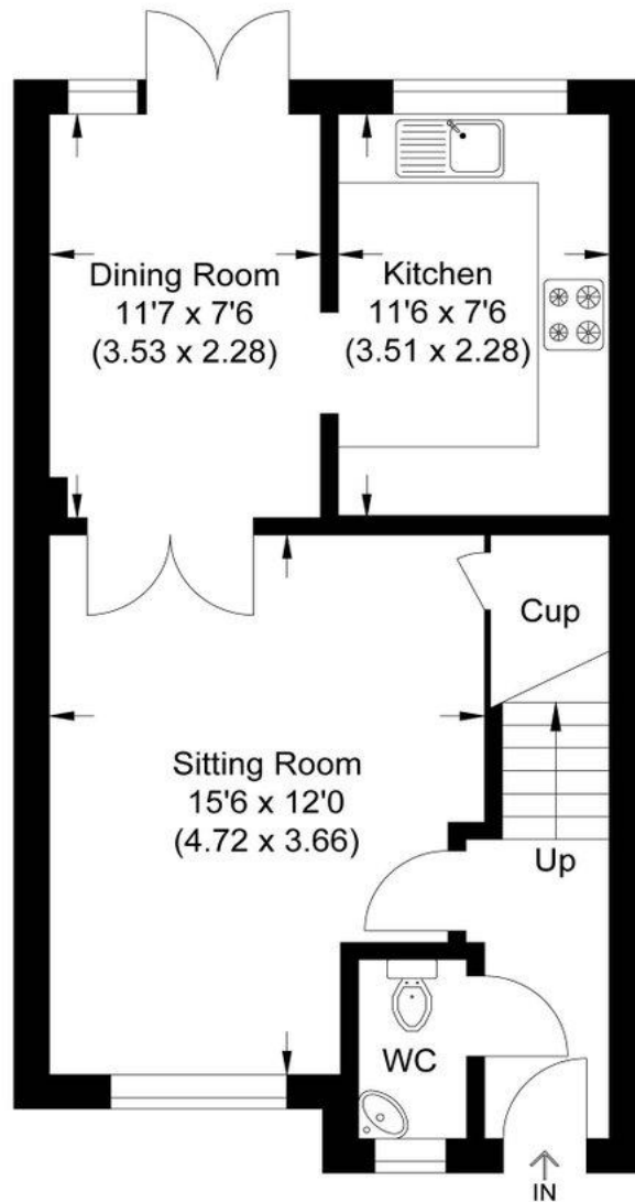
Ground Floor
