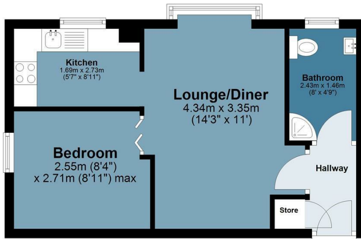
Ground Floor Approx. 29.6 sq. metres (319.1 sq. feet)
