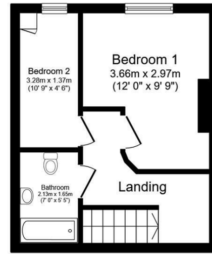
First Floor Floor area 23.9 sq.m. (258 sq.ft.)
