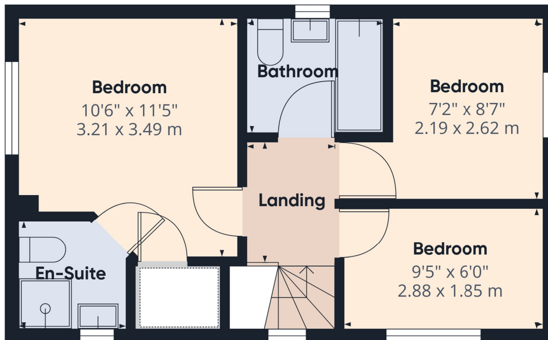
Floor 1 Building 1
