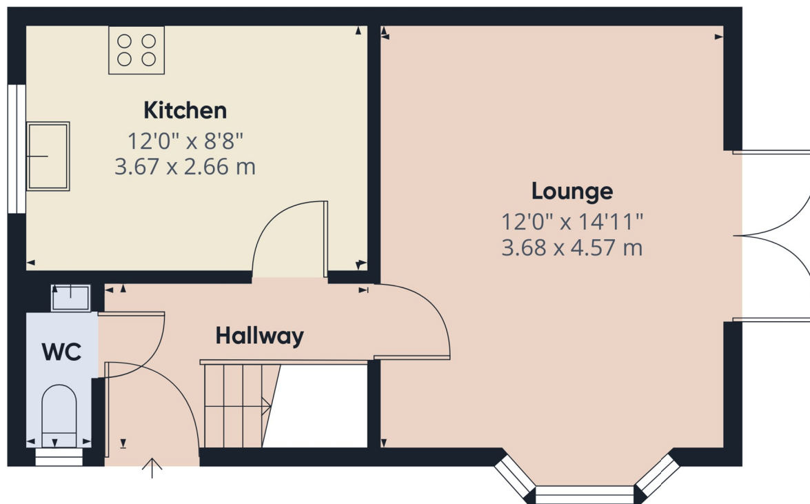
Floor 0 Building 1
