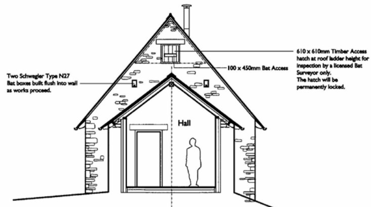
North Sectional Elevation B-B As Proposed
