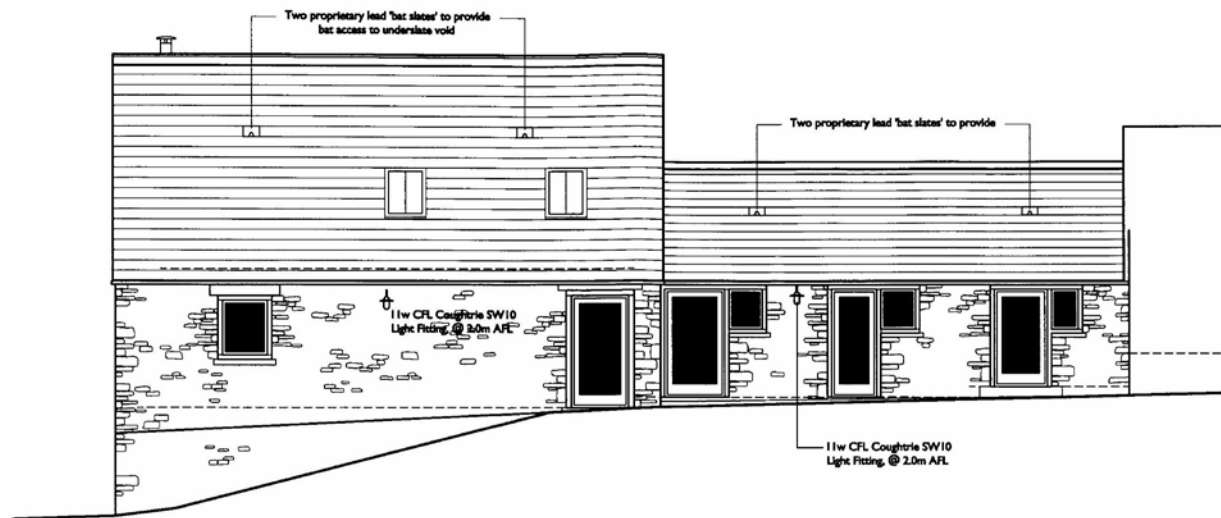
East Elevation As Proposed
