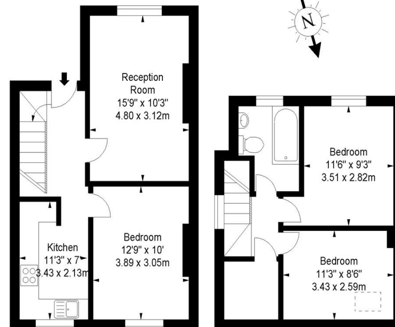
Second Floor
