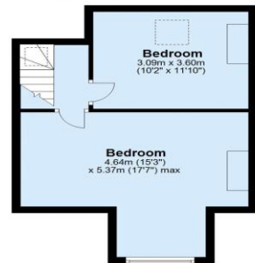
Second Floor Approx. 35.5 sq. metres (381.7 sq. feet)
