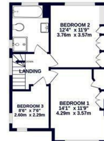
1ST FLOOR 538 sq.ft. (50.0 sq.m.) approx.
