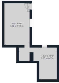
Floor -1 Building 1
