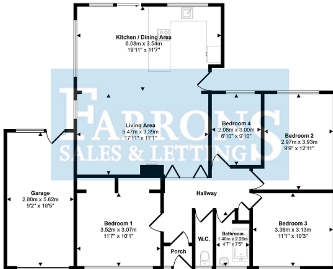
Floorplan
