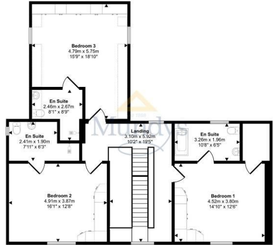
First Floor Approx 106 sq m / 1145 sq ft
