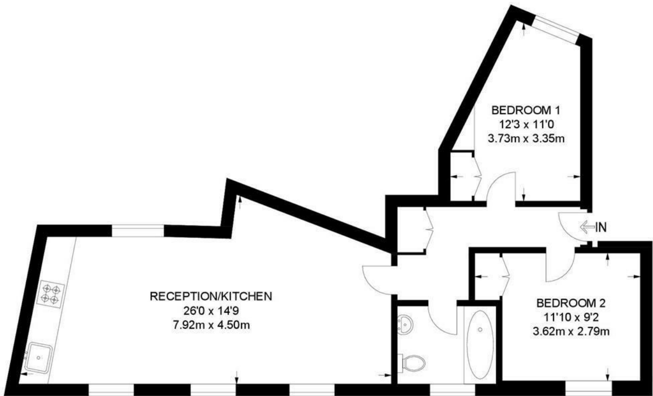
FIRST FLOOR
