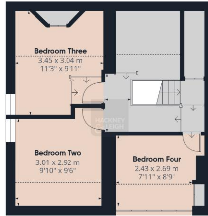
Floor 1 Building 1
